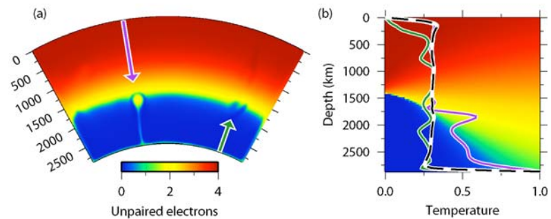
Figure 1. (a) Spin-state from simulation based on Sturhahn et al. (2005) spin model. Purple line is warm geotherm, green line is cold. (b) Geotherms with Sturhahn et al. (2005) spin-state model. Black dashed line is horizontal average.
